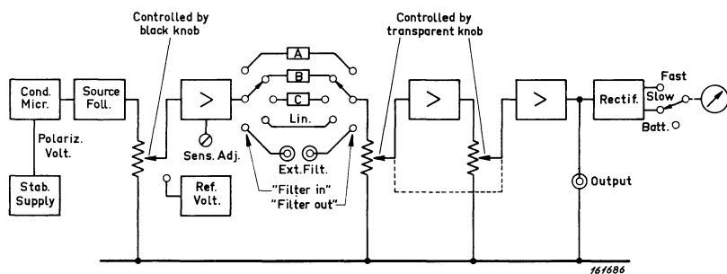
Fig. 2.2. Block diagram of Type 2203.
