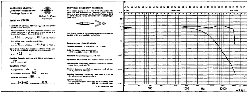
Fig. 5.1. Typical calibration chart as supplied with the microphone cartridges. The automatic plotting process used in production has an accuracy of 0.2 \text{ dB} up to 10 \text{ kHz} and 0.5 \text{ dB} up to 20 \text{ kHz} .
