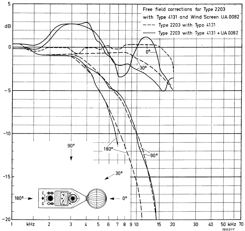
Fig. 8.9. Correction curves for 0°, 30°, 90° and 180° angles of incidence.
