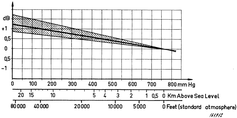
Fig. 5.2. Microphone sensitivity at 400 \text{ Hz} as a function of the static ambient pressure. The corresponding altitudes are also given on the curve.
