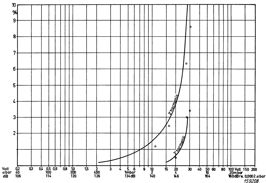
Fig. 5.9. Typical distortion curves for the one-inch microphones. The curves in full are measured on the source-follower and referred to a complete microphone with a sensitivity of 5 \text{ mV}/\mu\text{bar} . The measuring points shown are averages measured in a pistonphone on a number of complete microphones at 50 Hz.
